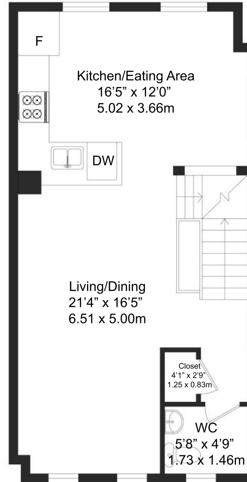
MAIN FLOOR 542 ft 2
